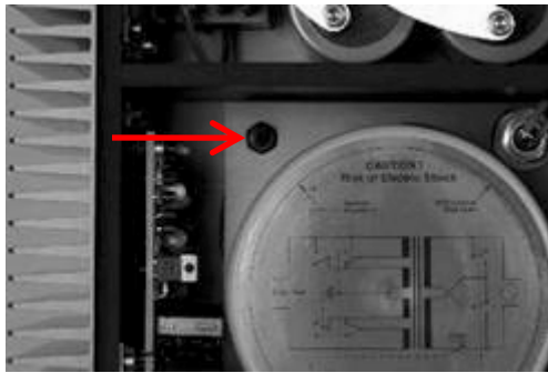
Fig.2 Speaker's impedance switch
